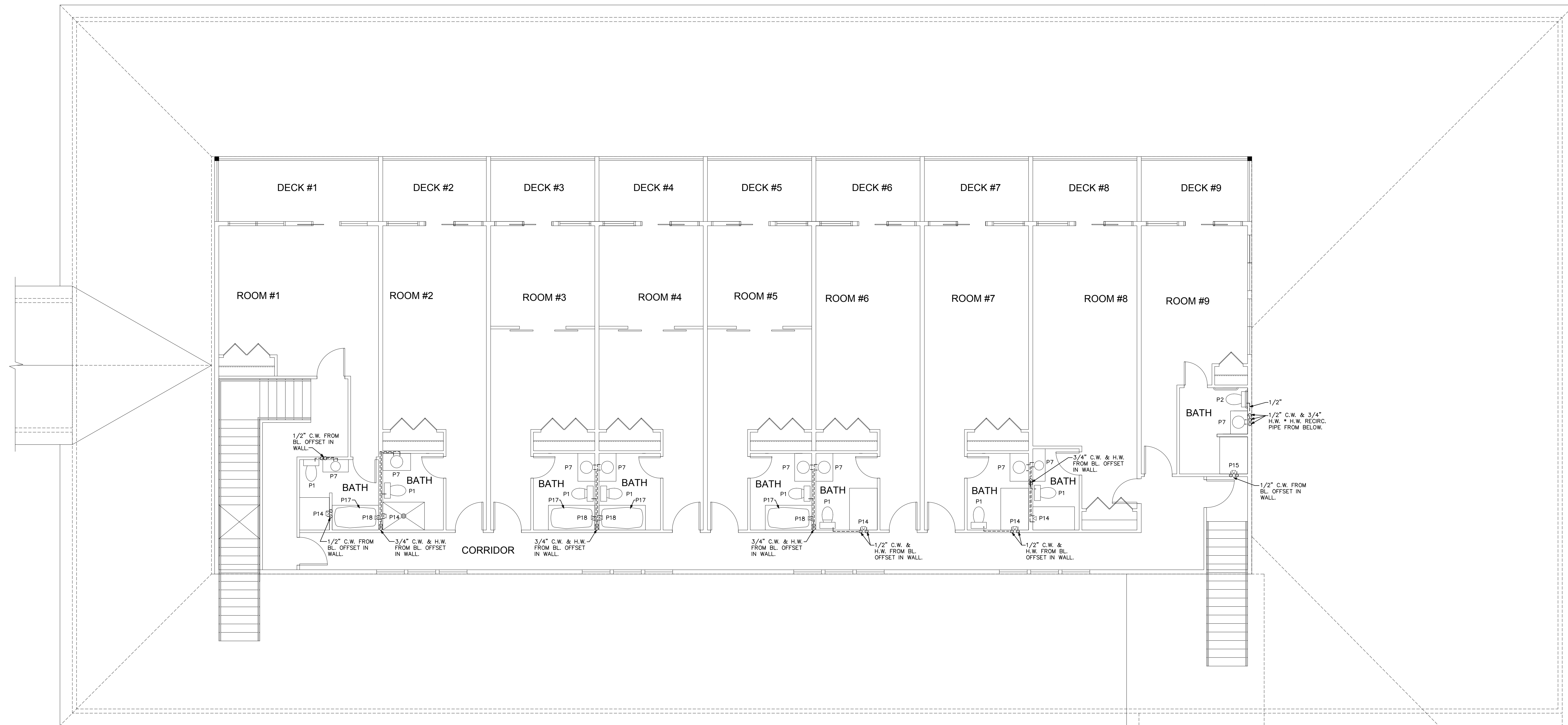
(WATER PIPING) 1 2ND LEVEL FLOOR PLAN - PLUMBING SCALE: 3/16"=1'-0"
