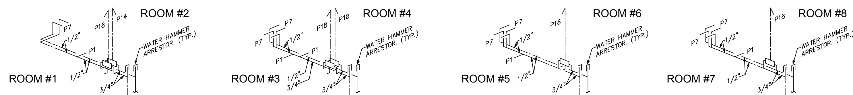
2 PARTIAL WATER PIPING ISOMETRICS NO SCALE
