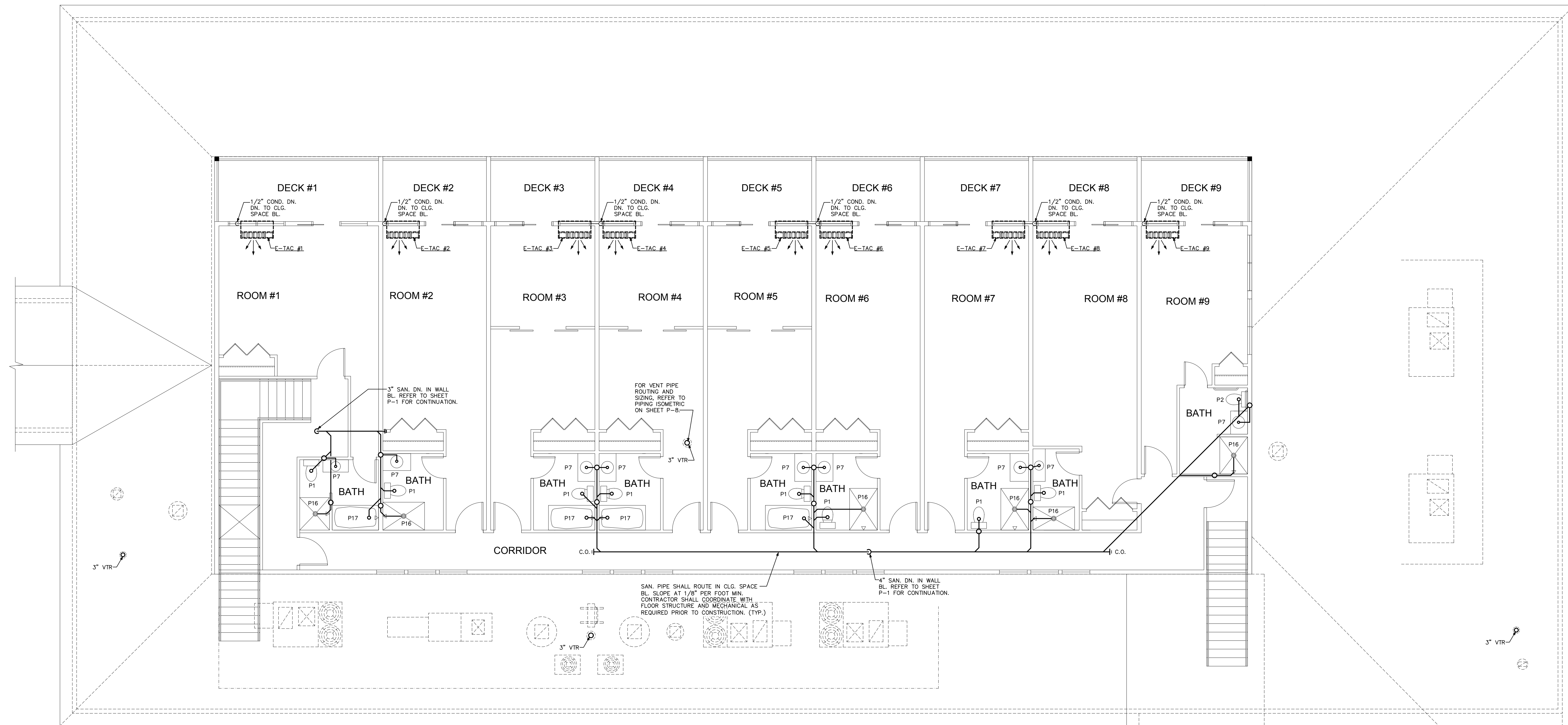
(SANITARY PIPING) 1 2ND LEVEL FLOOR PLAN - PLUMBING SCALE: 3/16"=1'-0"
